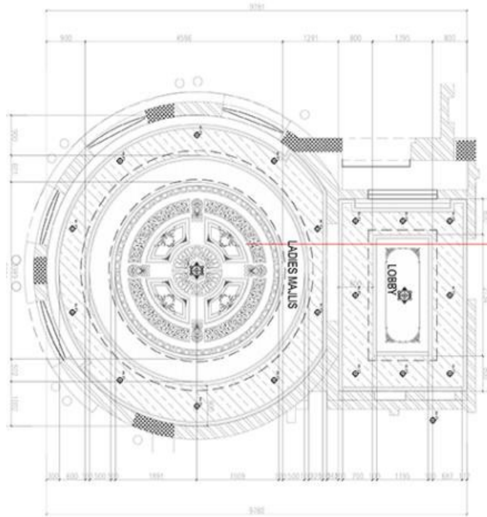
LADIES MAJLIS CEILING DESIGN
